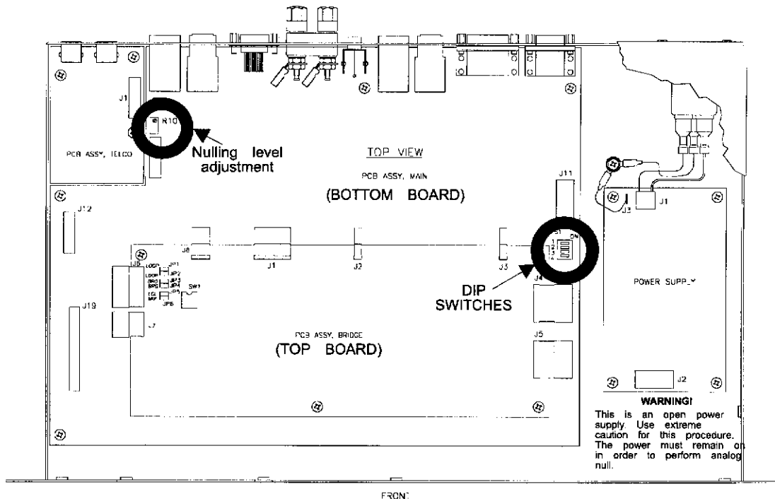
Figure 31. G3200 jumper locations
