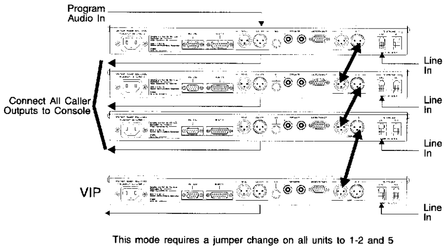
Figure 5a. G3200 VIP application with jumper changes
